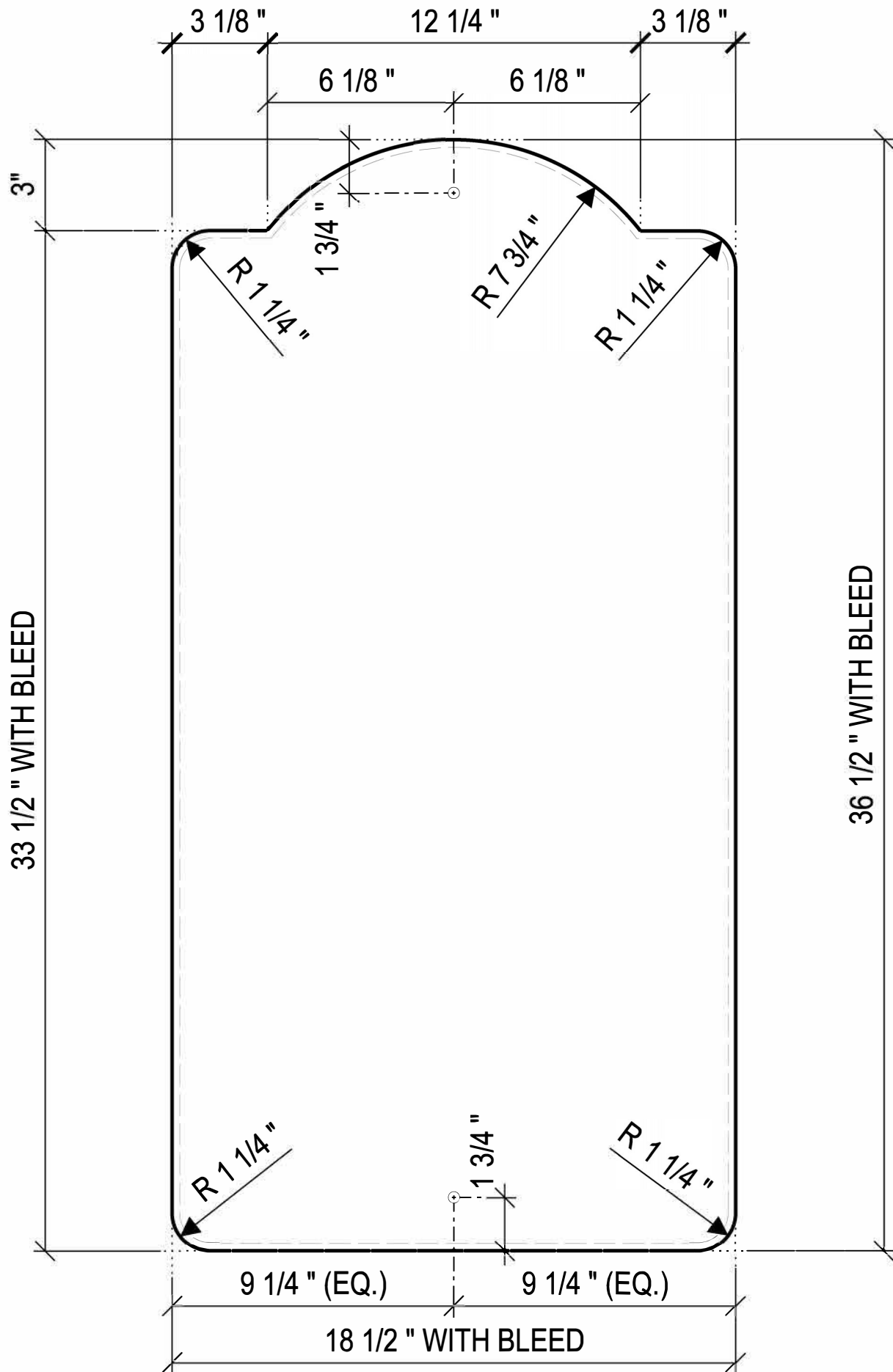
DIMENSIONS OF OVERPRINT COPY WITH \frac{1}{4} " BLEED
